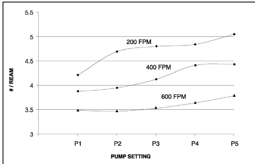
Coatweight vs. Linespeed vs. Pressure
